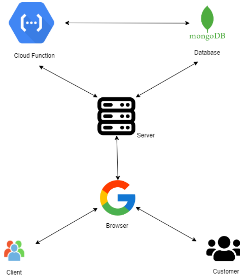
Figure 5.1: System Architect
