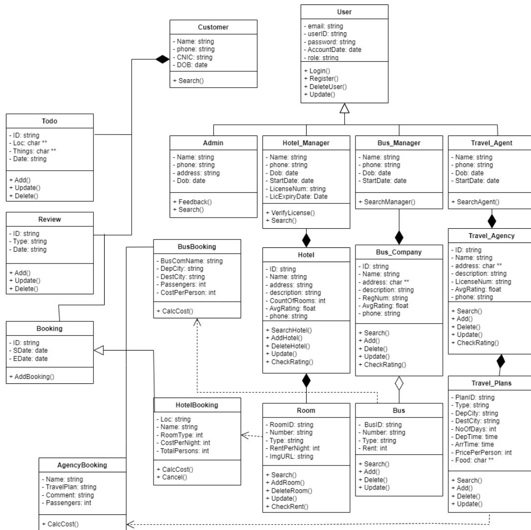
Figure 5.3: UML Class diagram
