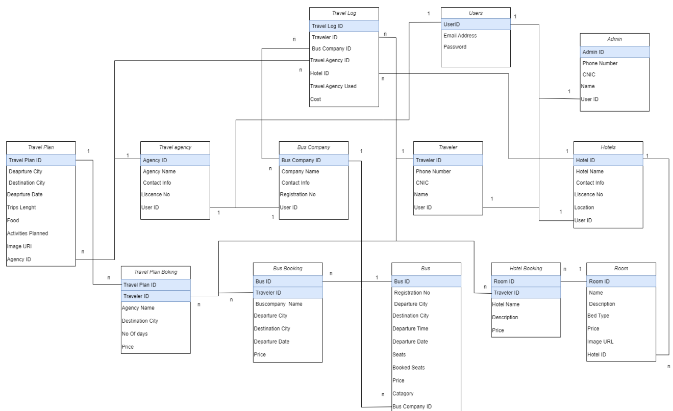
Figure 4.5: ER diagram of Rahzil
