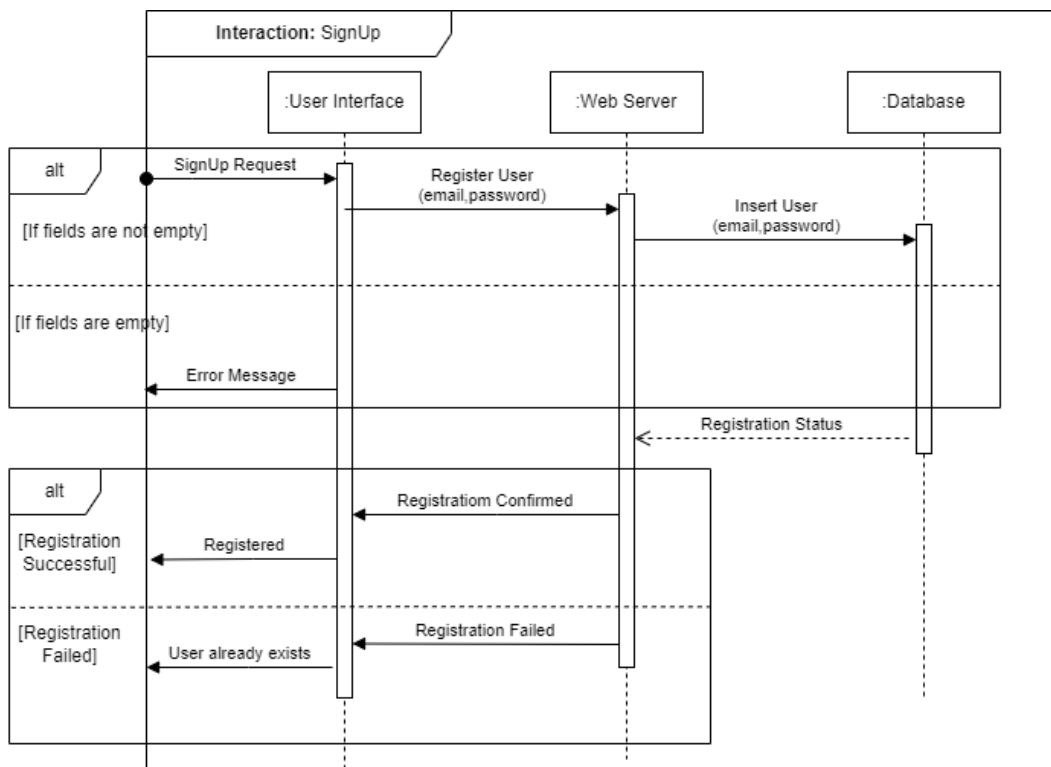
Figure 5.6: Client/Customer signup
