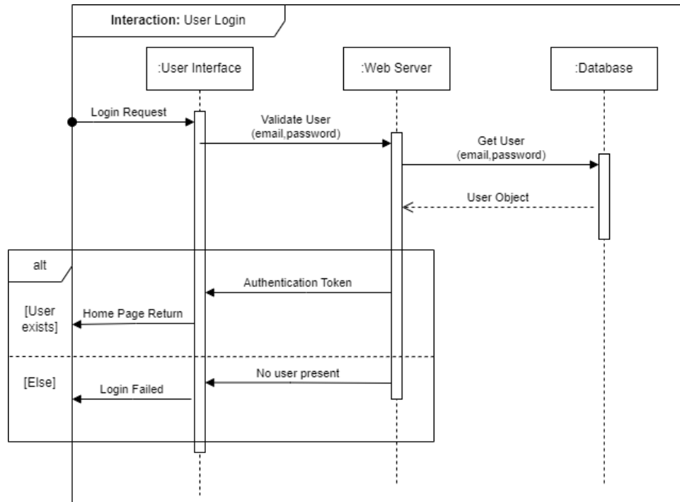
Figure 5.4: User Identification Sequence Diagram
