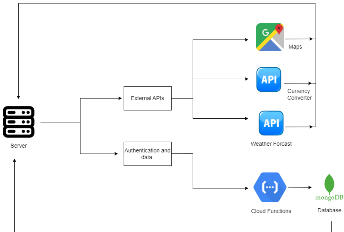
Figure 5.2: Subsystem Architect
