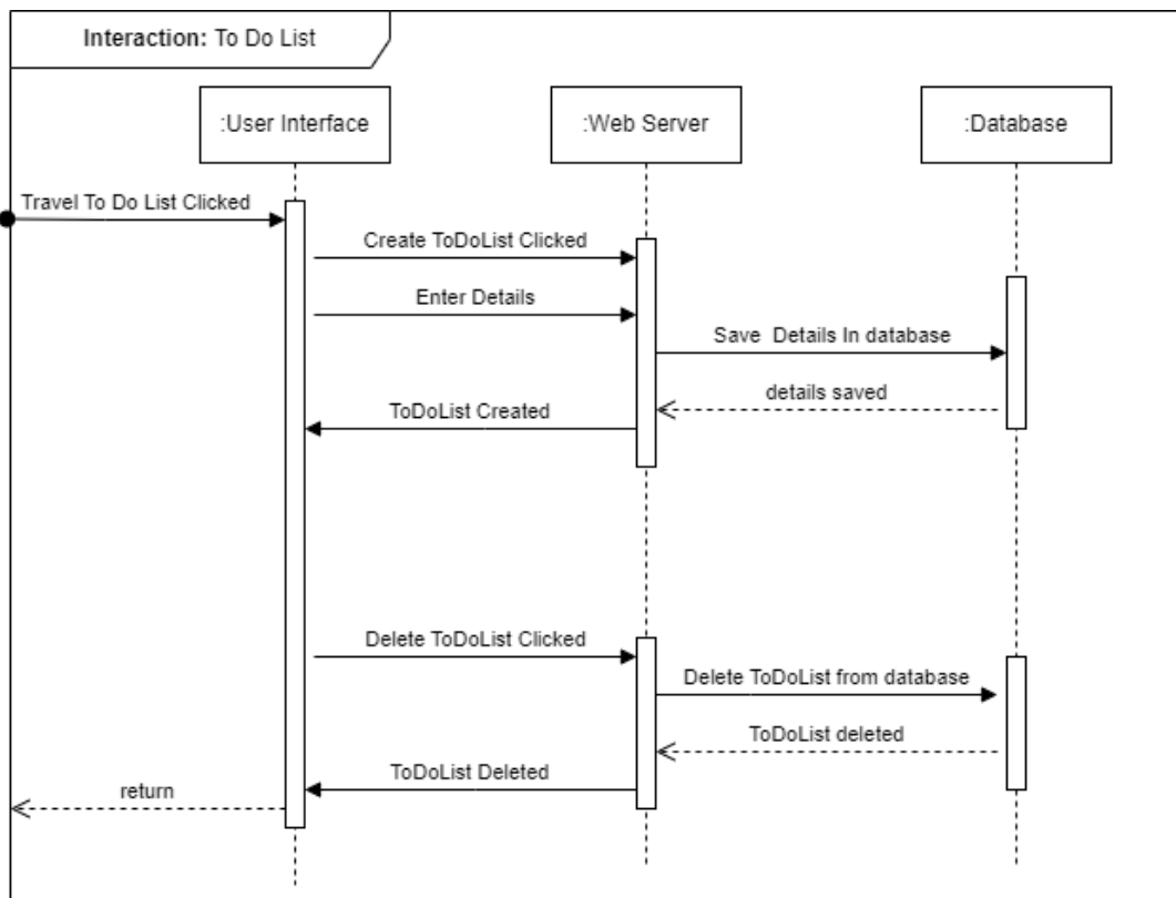
Figure 5.7: ToDo List
